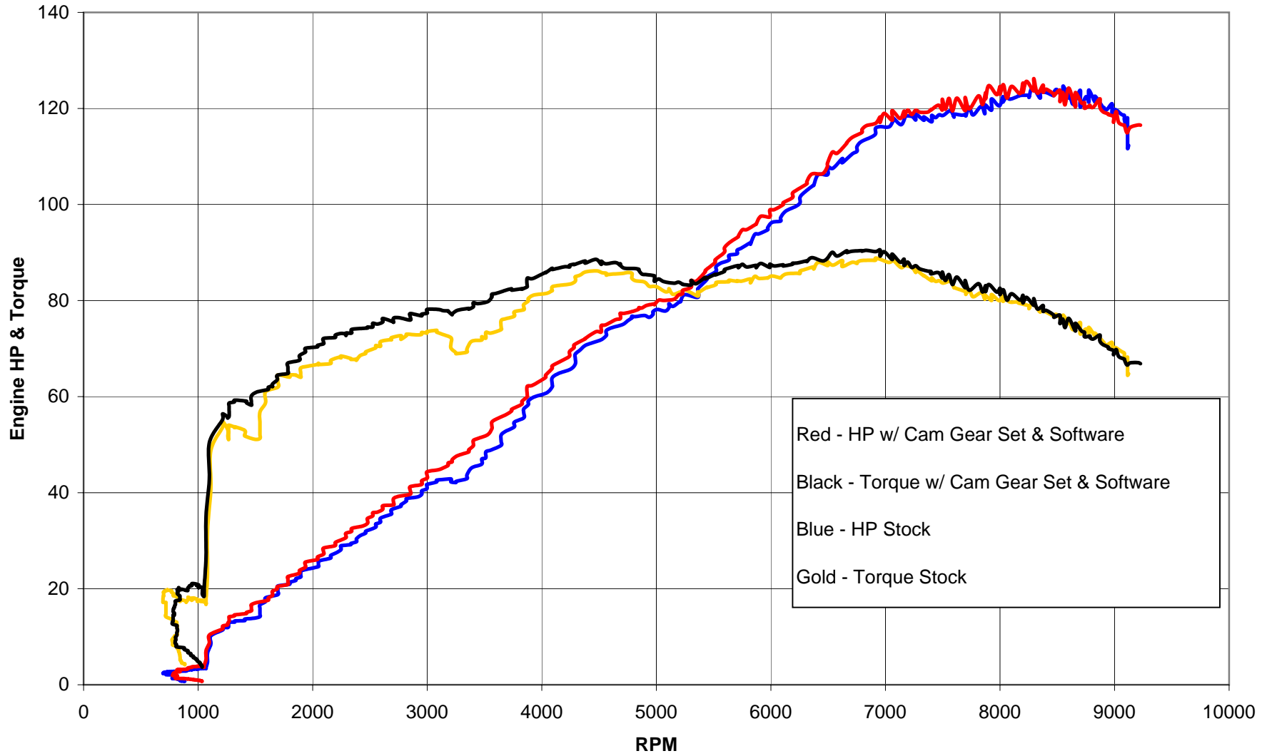
K1200rs/gt Stock vs. Cam Gear Set with Software
